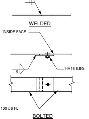
TYPICAL KICKPLATE SPLICE (N)
