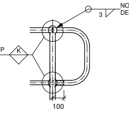
TYPICAL CLOSURE HANDRAIL JOINT (Q)
