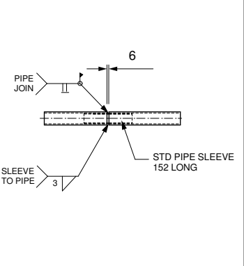
TYPICAL HANDRAIL SPLICE (P)
