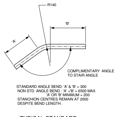
TYPICAL STANDARD & NON STANDARD ANGLE BENDS (M)
