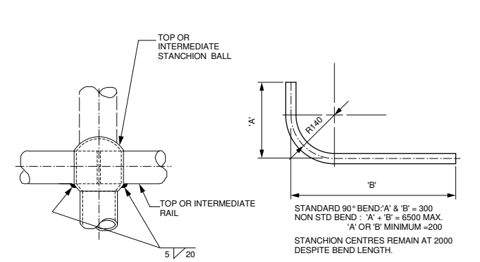
TYPICAL STANCHION/HANDRAIL JOINT (K)
